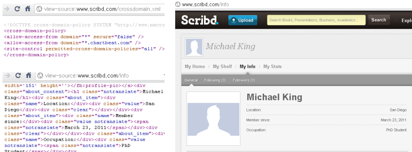
Figure 4. Crossdomain policy on www.scribd.com (Upper left), the content of a user’s information page (Lower left), and the screenshot of the page (Right).
